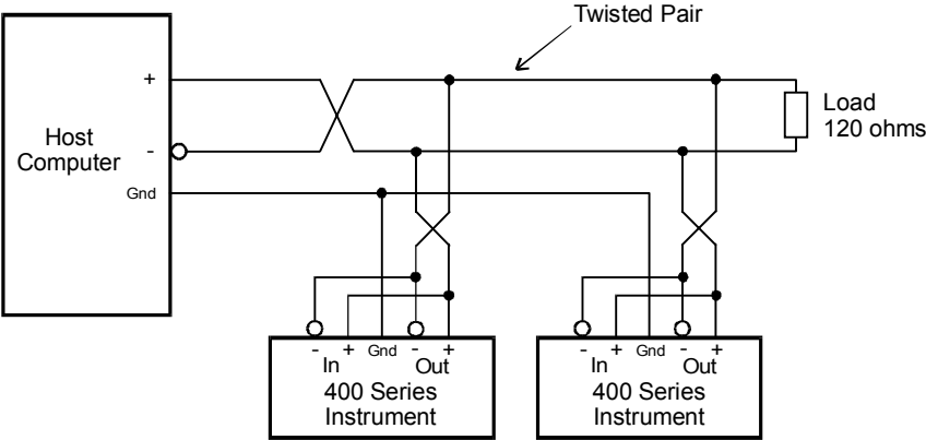
Figure 2 RS485 Interface
