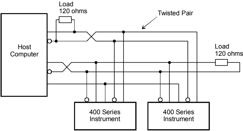
Figure 1 RS422 Interface
