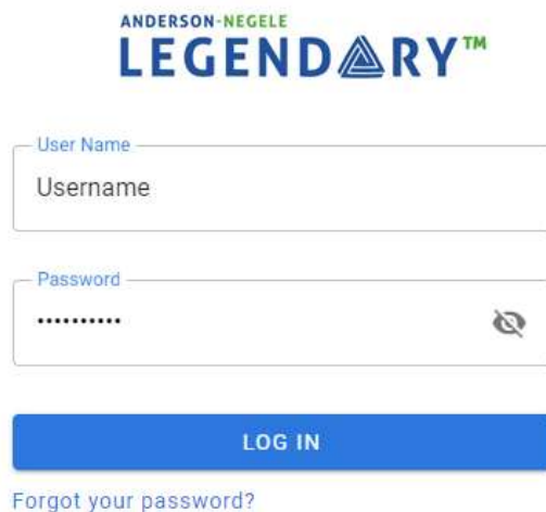
Figure 1: Legendary™ Login
