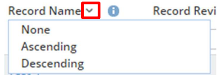
Figure 4: Sorting Records
