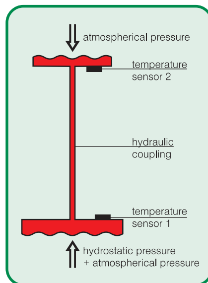
Fig. 2: Hermetically closed double membrane of the LAR-361
