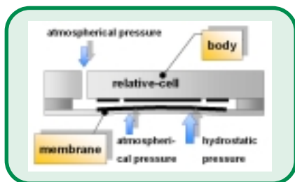
Fig. 1: Principle of Relative pressure cell
